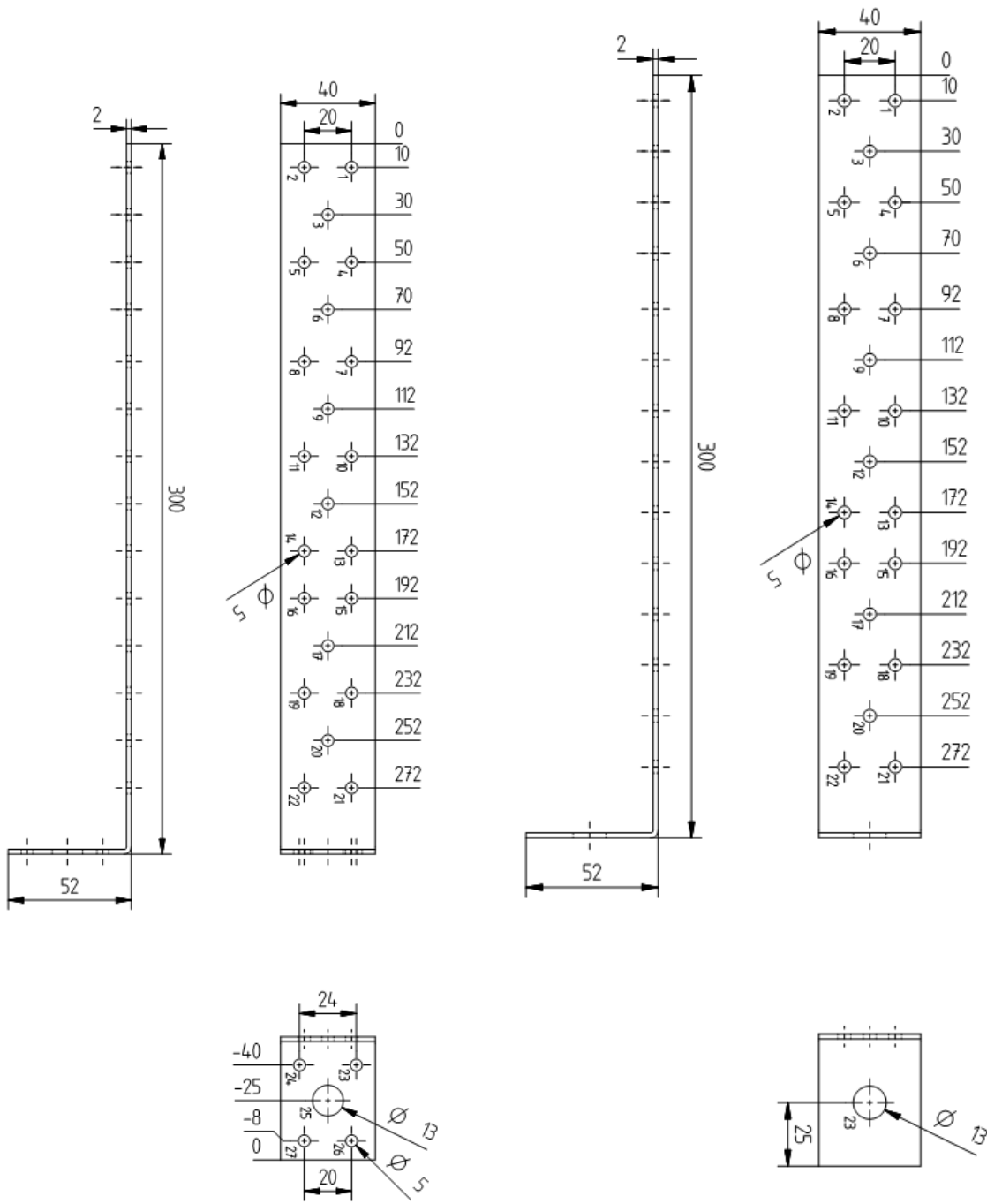
Figure A.67 hold-down 8795 3002 1D
